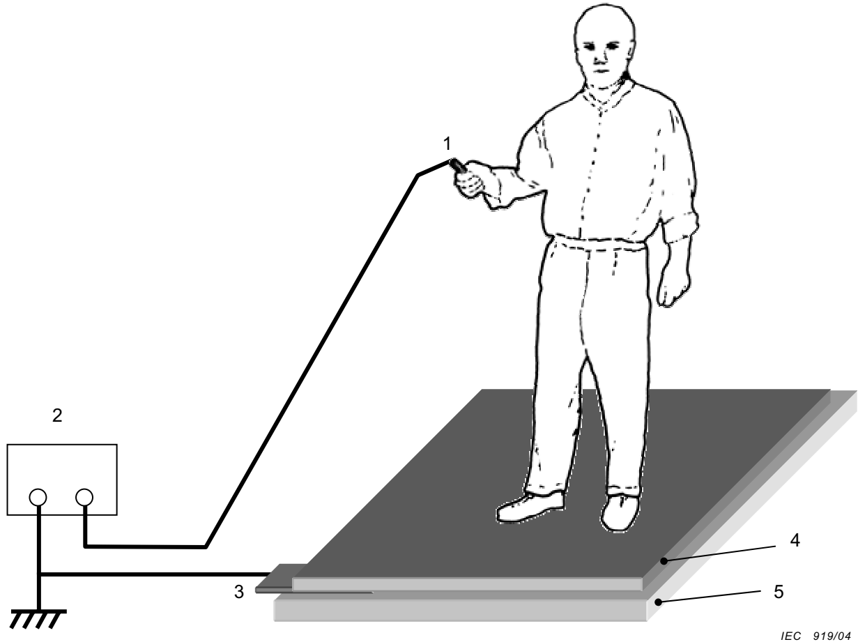
Figure 1a – Laboratory set-up
